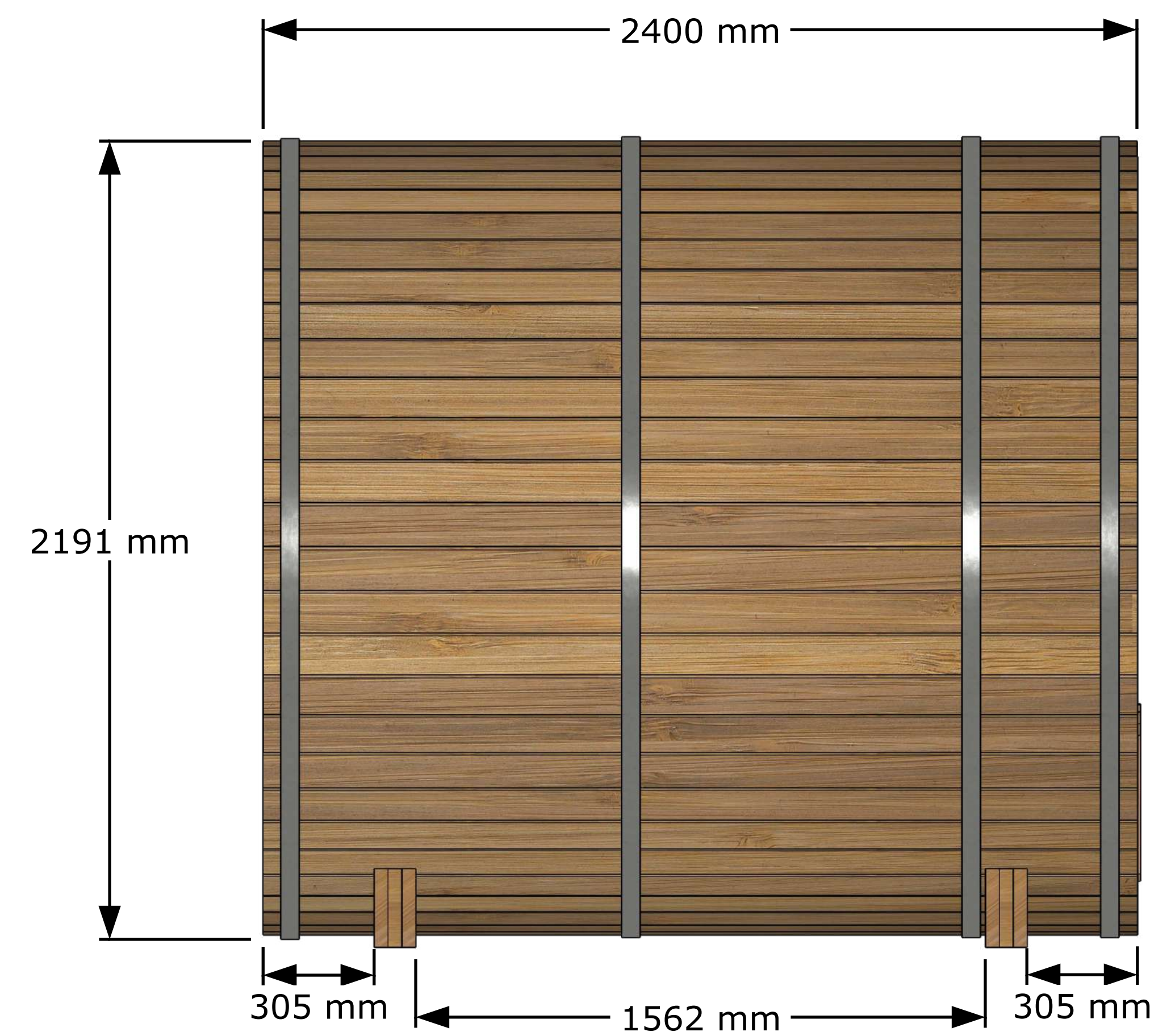
Side View
